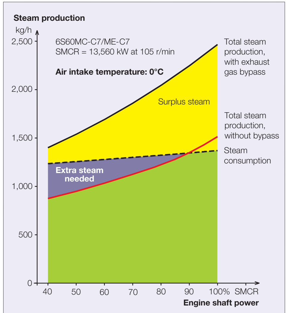
Fig. 12: Expected steam production by exhaust gas boiler at winter ambient conditions (0°C air) for main engine 6S60MC-C7/ME-C7 with/without a load-dependent low air temperature exhaust gas bypass system
