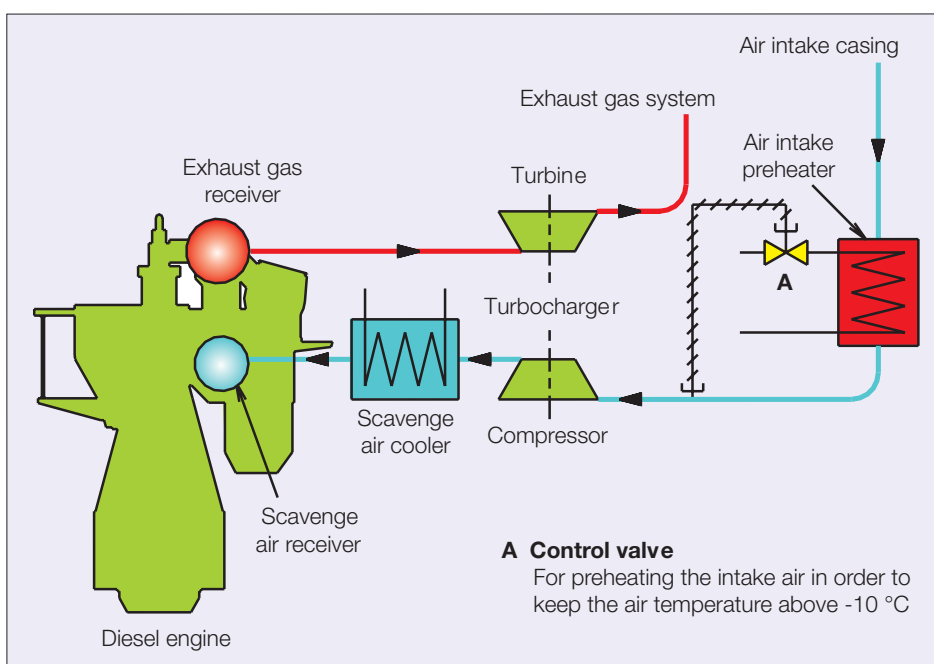
Fig. 8: Preheating of intake air
