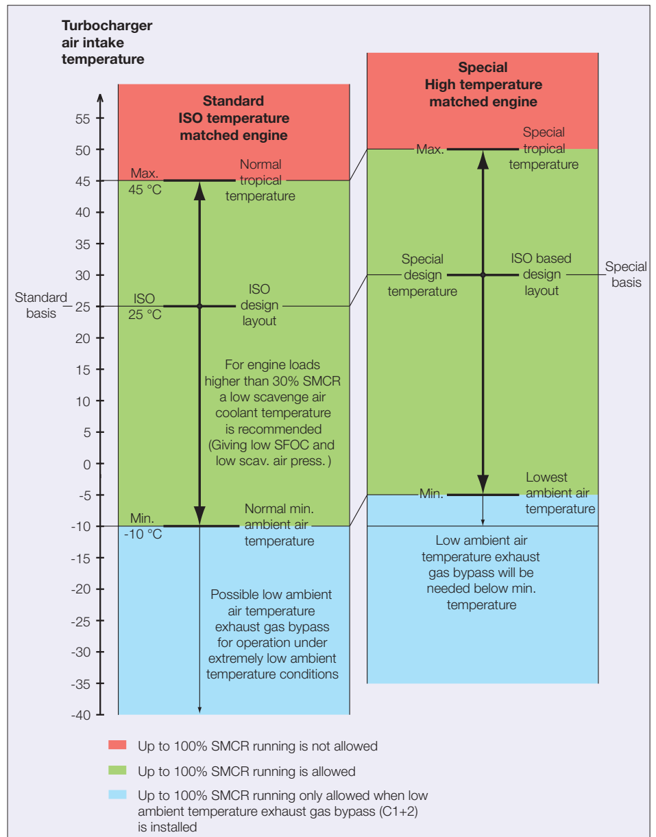
Fig. 7a: Principles for standard and special high ambient air temperature matched engine
