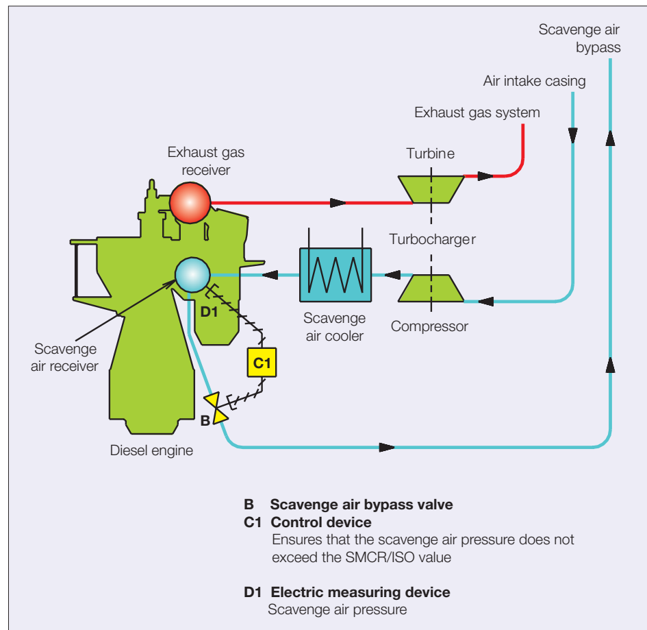
Fig. 9: Scavenge air bypass system
