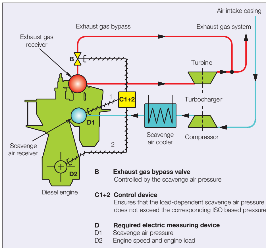
Fig. 10: Standard load-dependent low ambient air temperature exhaust gas bypass system
